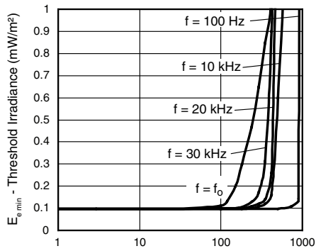
20746 \Delta V_{RMS} - AC Voltage on DC Supply Voltage (mV)
